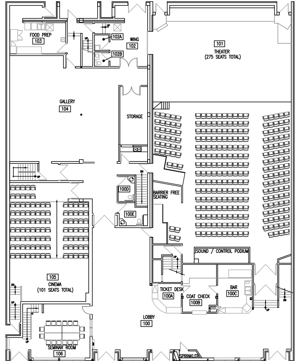
1 MAIN FLOOR PLAN A1 JANUARY/2017
